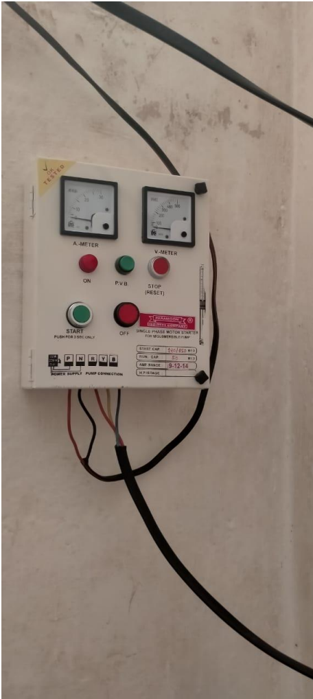
Electricity connection repair and wiring in 02 NGs of Balod-Sanjari 01 and Kotera 03. Meter was rewired followed by pipe connection.
